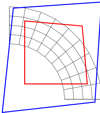
Figure 6. Central torsional kernel for the original configuration (inner kernel) and the optimized one (outer kernel).
