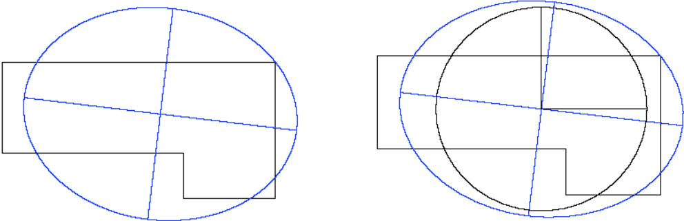
Figure 2. Comparison between the Cullman Ellipses in the first and last floor.
