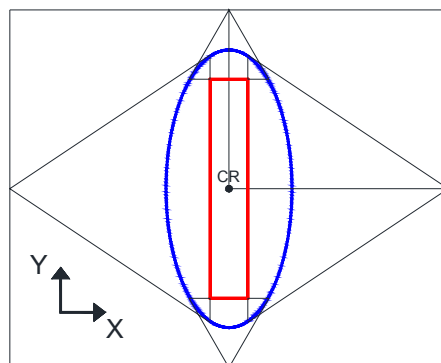
Figure 9. Central torsional kernel for the Cullman ellipse of figure 7
