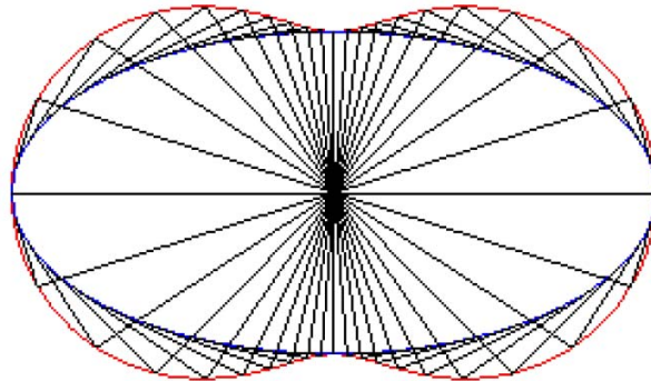
Figure 12. Relationship between a Booth curve and its inscribed Ellipse, and its 4 common points, at the extremities of each semi axis.
